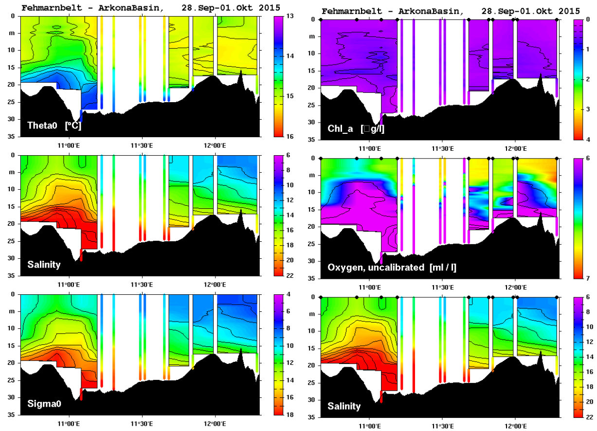
Figure 4.2: Potential temperature, salinity and potential density distribution along zonal section between 28. and 30. Sept. 2015.
