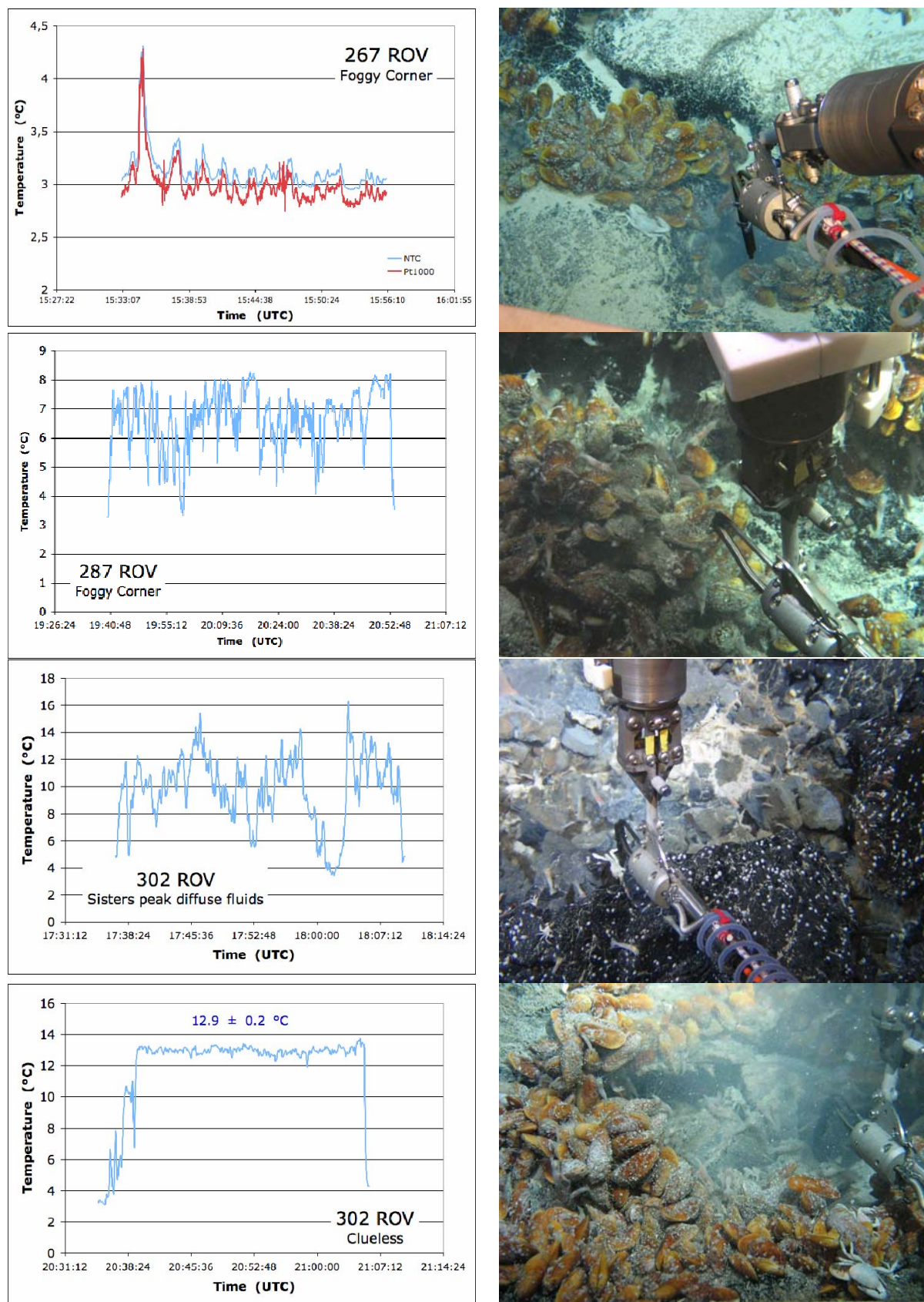
Fig. 3: Temperature logs during KIPS sampling of diffuse hydrothermal fluids in musselfields at 5 °S MAR, Comfortless Cove: Foggy Corner (267 ROV, 287 ROV), Sisters Peak and Clueless (302 ROV).
