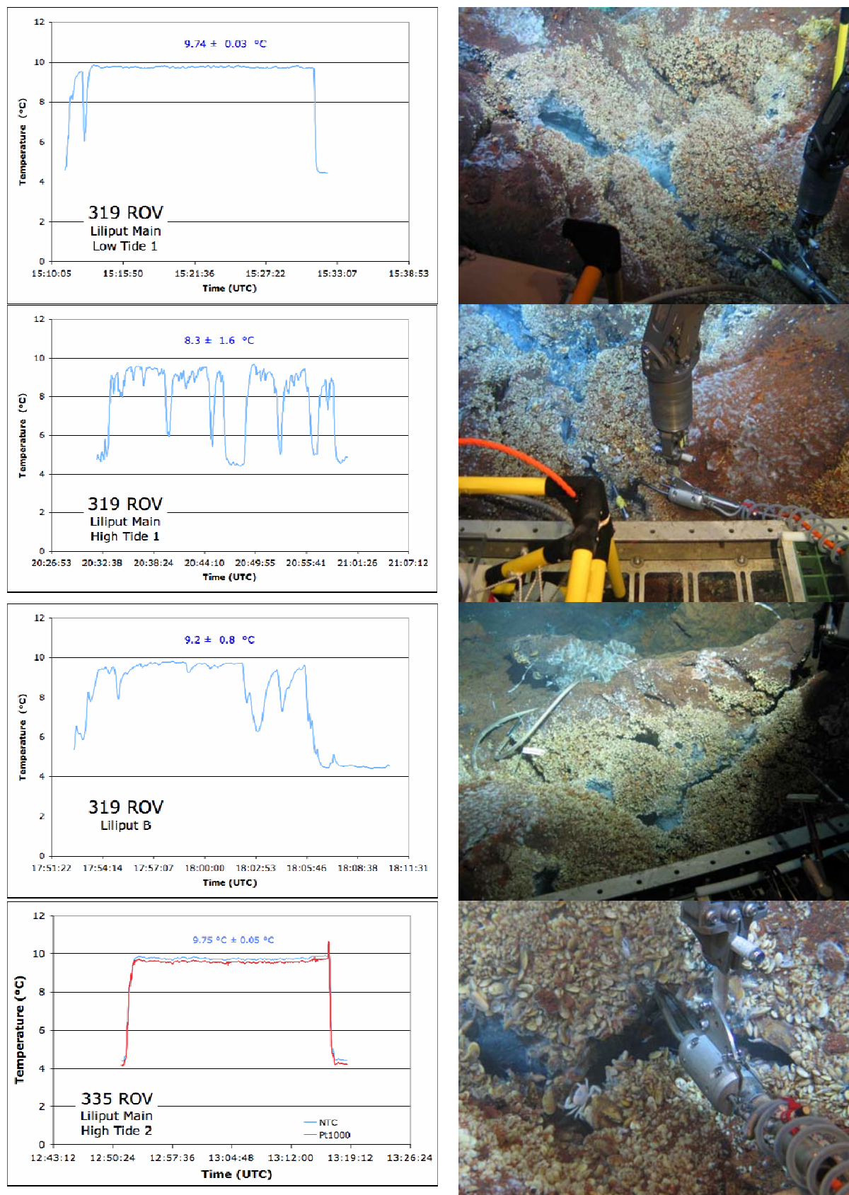
Fig. 4: Temperature logs during KIPS sampling of diffuse hydrothermal fluids in musselfields at 9°55 S MAR, Liliput Main (319 ROV and 335 ROV).
