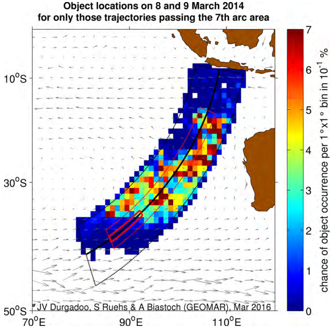
Figure 6: Locations on 8 and 9 March 2014 of only those objects that were within 5^\circ on either side of the 7 th arc (as in Figure 4) and reached La Réunion within the period 1–28 June 2015. The colour shading shows the object location counts per 1^\circ \times 1^\circ bin divided by the total amount of object location counts in the 7 th arc area (dashed black) on 8–9 March 2014 in %. It indicates the chance of objects occupying a particular bin on these two days; the values of all bins sum up to 100 %. The 7 th arc, wide and priority search areas are overlaid.
