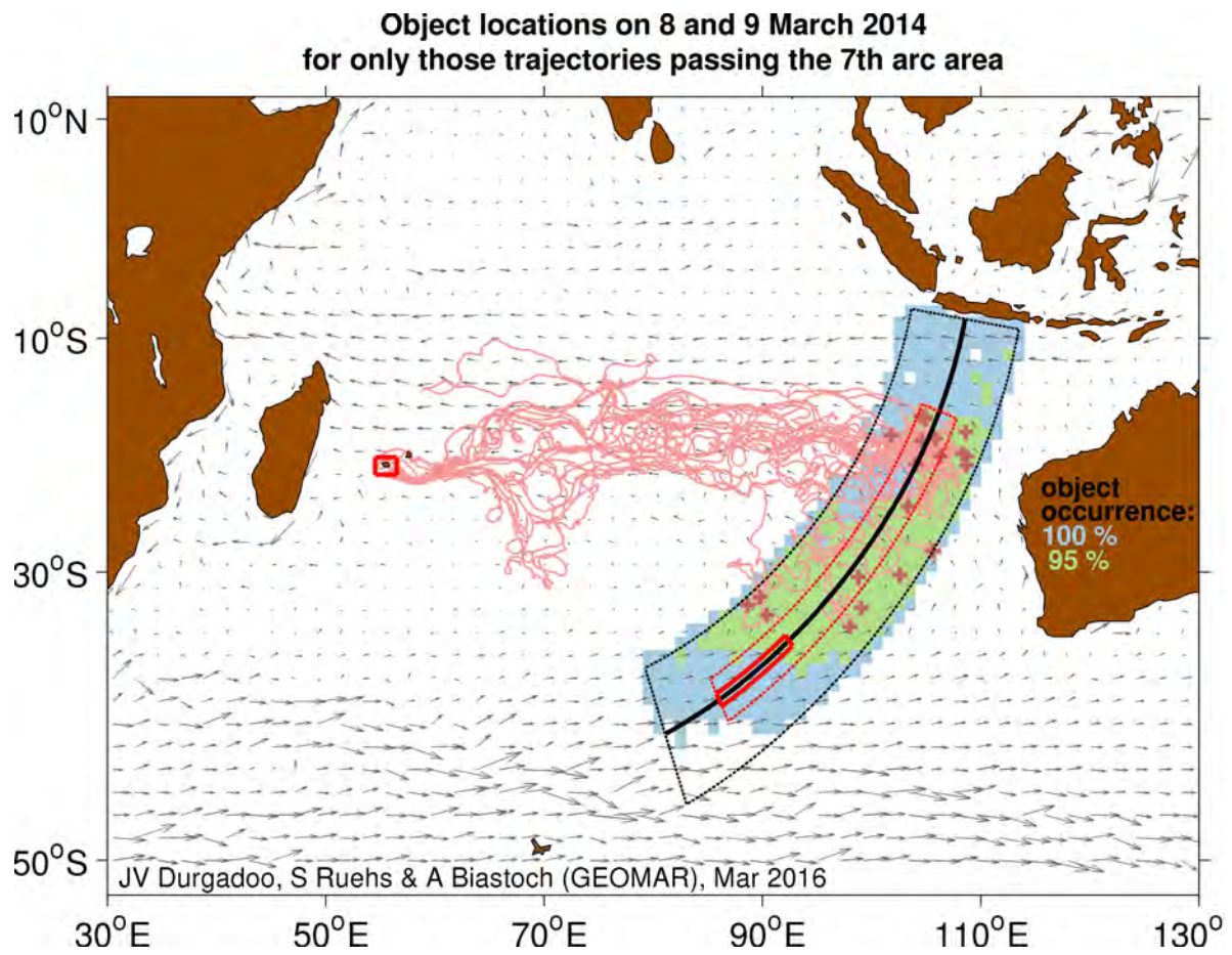
Figure 7: Most likely area where the flaperon found at La Réunion in July 2015 started its drift in the timeframe 8–9 March 2014. The chances of object occurrence displayed in Figure 5 were cumulated recursively above a certain threshold to determine the most likely start area encompassing 95 % of the object occurrences, shaded in green. Examples of possible drift trajectories of the flaperon are displayed in red. The 7 th arc, wide and priority search areas are overlaid.
