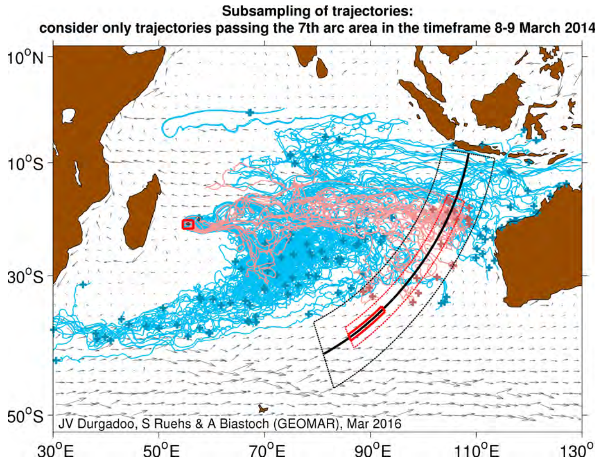
Figure 5: As Figure 3 but with highlighted (red colour) trajectories of those objects which were within 5° on either side of the 7 th arc (marked in dashed black) in the timeframe 8–9 March 2014.
