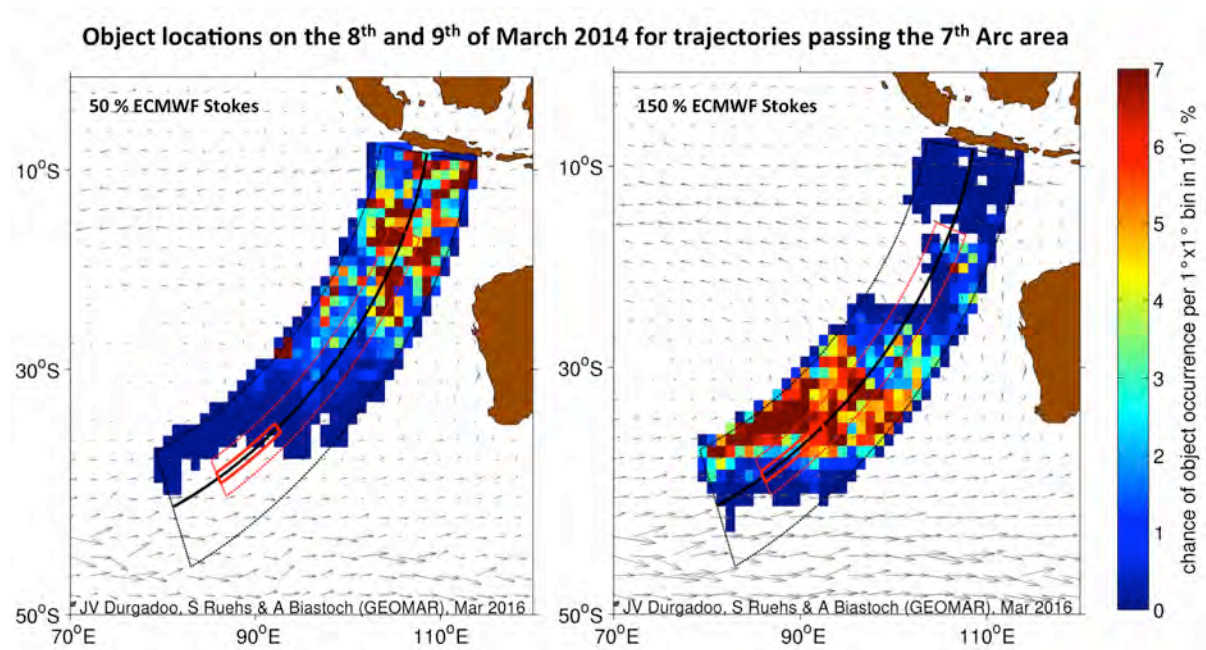
Figure A1: Locations on 8 and 9 March 2014 of only those objects that were within 5° on either side of the 7th arc and reached La Réunion within the period 1–28 June 2015. The colour shading shows the object location counts per 1° x 1° bin, divided by the total amount of object location counts in the 7th arc area (dashed black) on 8–9 March 2014 in %. It indicates the chance of objects occupying a particular bin on these two days; the values of all bins summing up to 100%. The 7th arc, wide and priority search areas are overlaid. Trajectories have been calculated by using surface currents based on CMEMS and 50% (left) and 150% (right) of the ECMWF Stokes drift.
