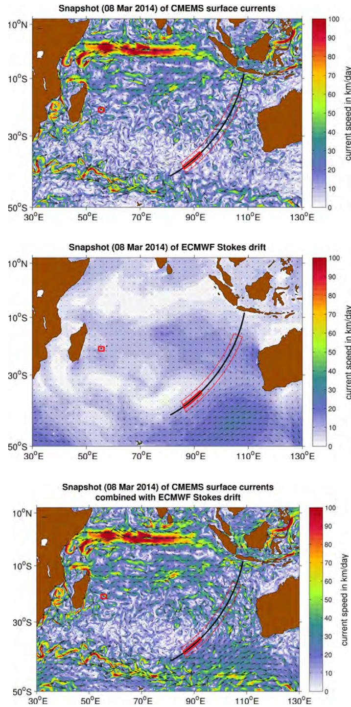
Figure 1: Snapshot for 8 March 2014, on the day MH370 went missing, of surface currents from the Copernicus Marine Environment Monitoring Service , upper row), Stokes drift ( European Centre for Medium-Range Weather Forecasts , middle row), and combination of both (lower row). Shown are direction (arrows shown every 2°) and speed (colour shading in km/day). The black arc indicates the possible location of the aircraft in the eastern Indian Ocean during its last successful automated satellite contact on 8 March 2014 (7 th arc). The red dashed framed area marks the wide underwater search area obtained from engine fuel consumption considerations (meridional extent defined in Table 2 of footnote 2); the red solid framed area indicates the current (defined December 2015) priority search area 3 . The island of La Réunion is highlighted by a small red square box.
