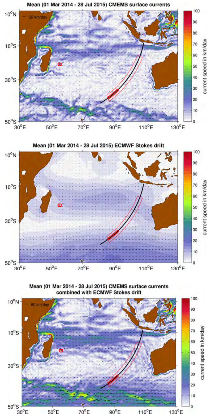
Figure 2: As Figure 1 but as average for the period 1 March 2014 – 28 July 2015
