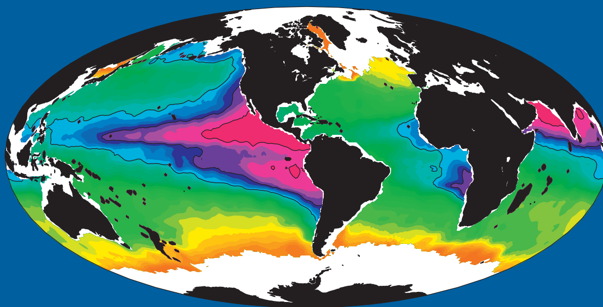
Dissolved oxygen concentrations on the 26.9 isopycnal (at a depth of about 300m). Pink areas denoting low oxygen waters are located predominantly in the tropical ocean.
