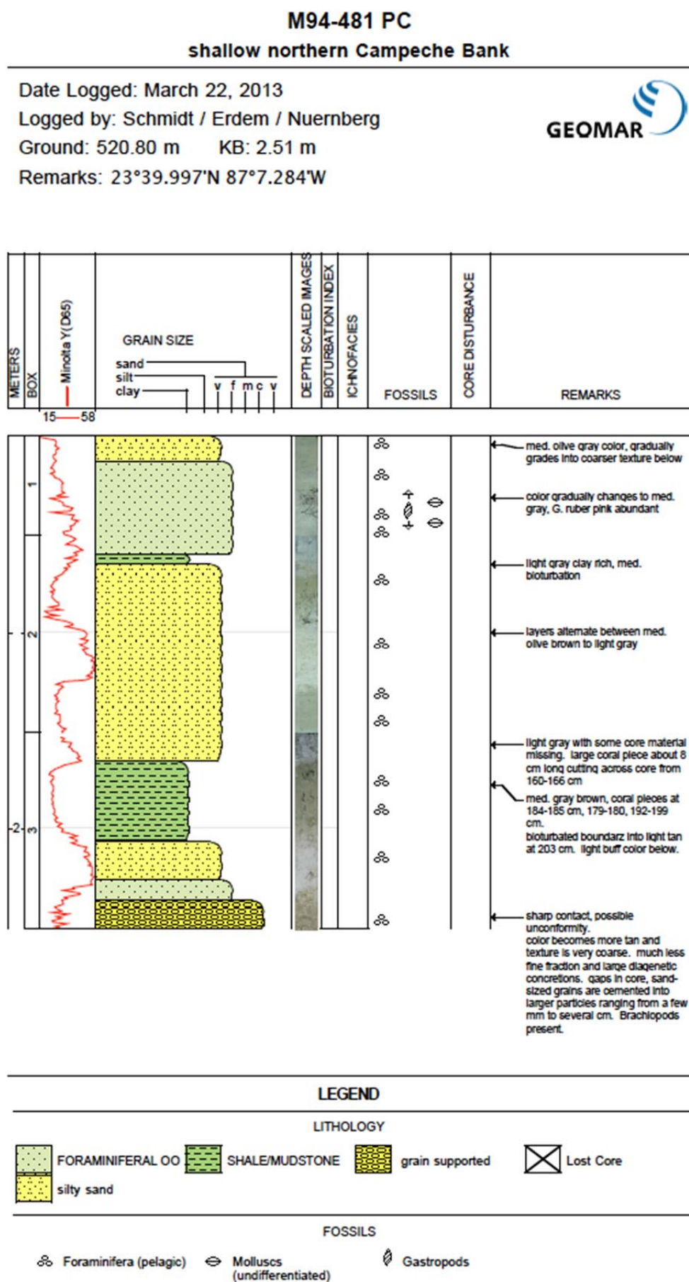
Fig. A11.1.7 Lithology log of core M94-481 Piston Core (by AppleCORE v10.2a).
