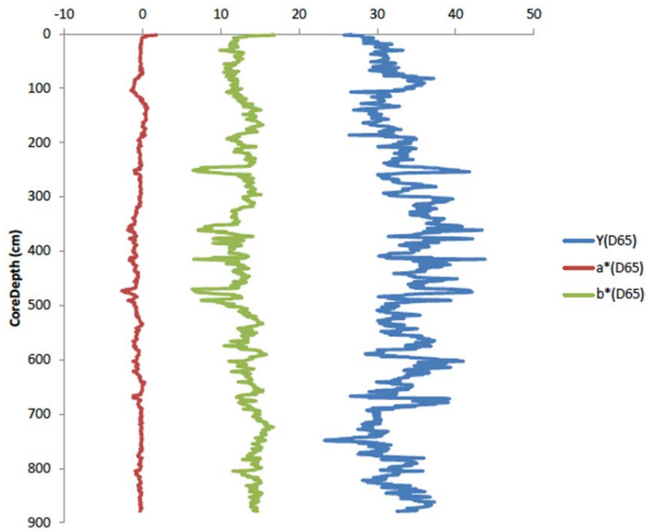
Fig. A11.3.7. Minolta color scanner data of core M94-482 PC from the northern Campeche Bank (23°49.155 N 87°7.752 W, 629 m water depth): Y (D65), a* and b* CIELAB color coordinates. The Y-values represent the lightness on a linear scale. The a*-values indicate the relationship between green and magenta and the b*-value reflects blue/yellow colors.
