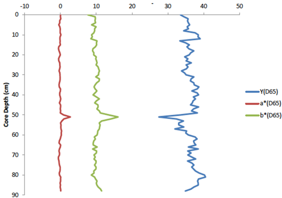
Fig. A11.3.2. Minolta color scanner data of pilot core M94-473 PC from Yucatan Strait (21°44.646 N 86°14.163 W, 933 m water depth): Y (D65), a^* and b^* CIELAB color coordinates. The Y-values represent the lightness on a linear scale. The a^* -values indicate the relationship between green and magenta and the b^* -value reflects blue/yellow colors.
