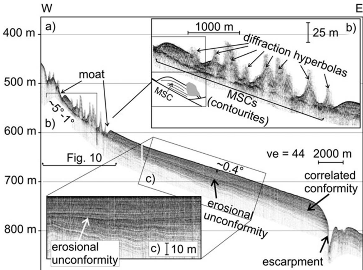
Fig. 5.2.3.3.1 PARASOUND section from the northeastern Campeche Bank from Hübscher et al. (2010). In water depths between 520 m and 600 m, a system of mounded sediment complexes (MSC) is present. Below and above a prominent escarpment, a layered sequence of sediments is present, with a correlated conformity in the lower part transforming into an erosional unconformity further upslope.
