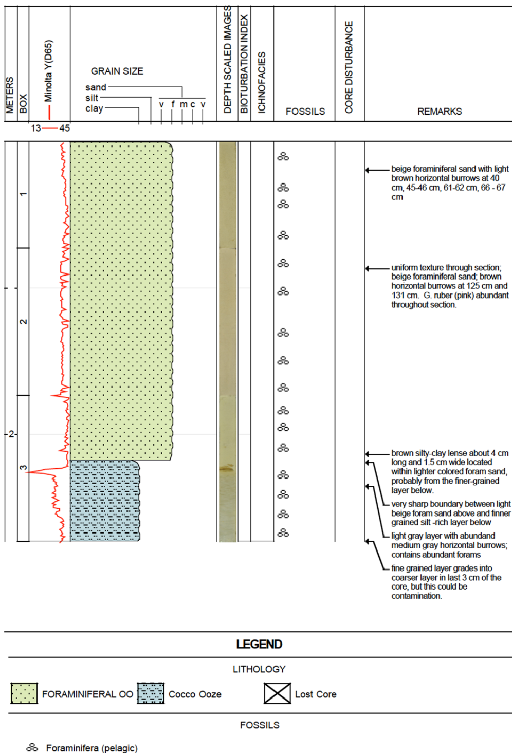
Fig. A11.1.2 Lithology log of core M94-473 Piston Core (by AppleCORE v10.2a).
