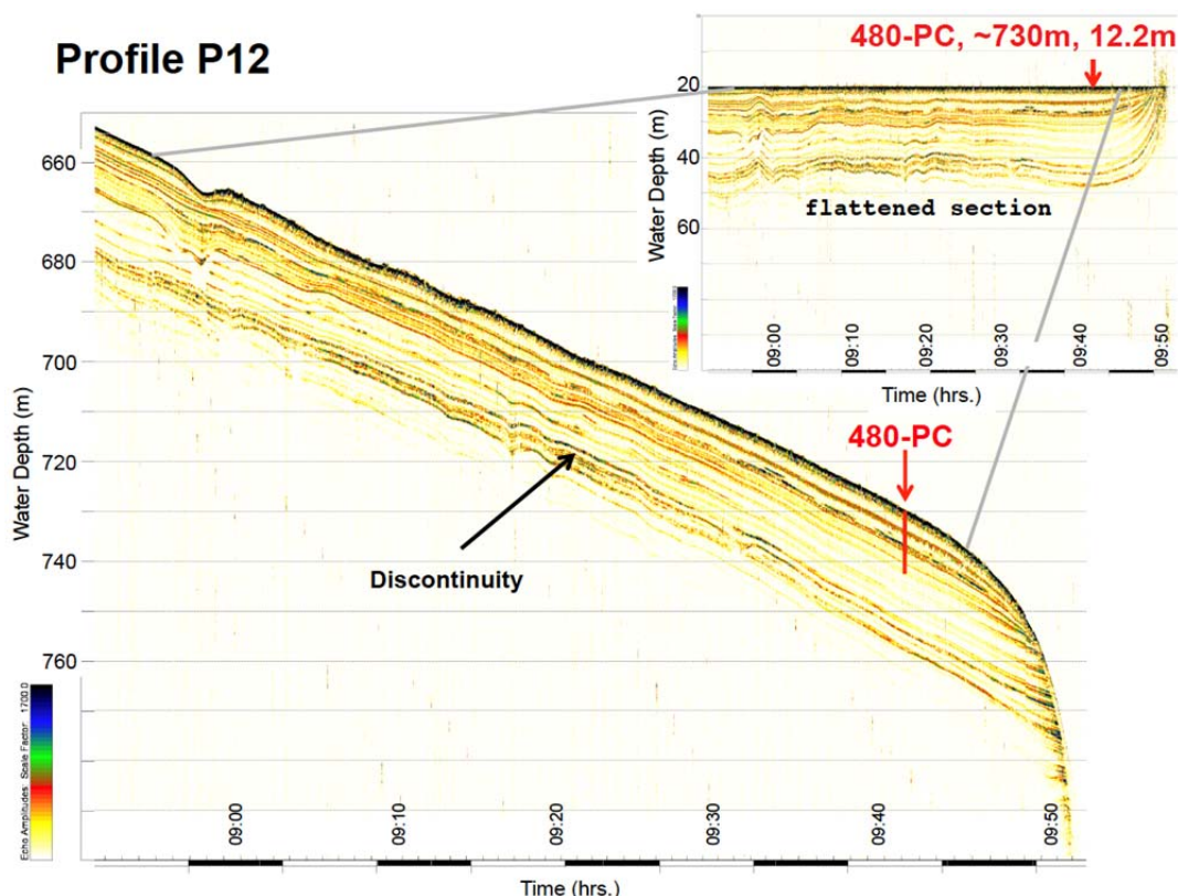
Fig. 5.2.3.3.2. West-east striking seismic profile (P12) that covers a seafloor depth range of ~650–800 m from the northern Campeche Bank, accomplished during M94. The locations of piston corer M94-480 PC (~730 m water depth, ~12.2 m core recovery) is indicated. Upper right inlet is the respective flattened section. For location see Fig. 5.3.2.1.
