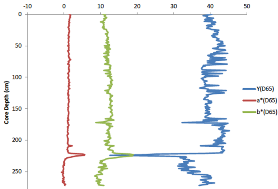
Fig. A11.3.1. Minolta color scanner data of core M94-473 PC from Yucatan Strait (21°44.646 N 86°14.163 W, 933 m water depth): Y (D65), a^* and b^* CIELAB color coordinates. The Y-values represent the lightness on a linear scale. The a^* -values indicate the relationship between green and magenta and the b^* -value reflects blue/yellow colors.
