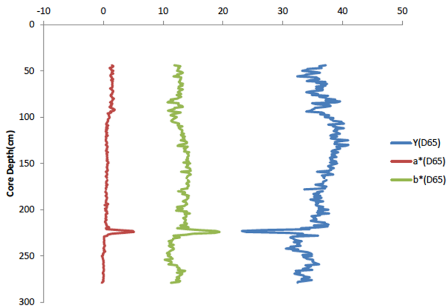
Fig. A11.3.3. Minolta color scanner data of core M94-475 PC from Yucatan Strait ( 21^{\circ}46.277 N 86^{\circ}16.084 W, 767 m water depth): Y (D65), a^* and b^* CIELAB color coordinates. The Y-values represent the lightness on a linear scale. The a^* -values indicate the relationship between green and magenta and the b^* -value reflects blue/yellow colors.
