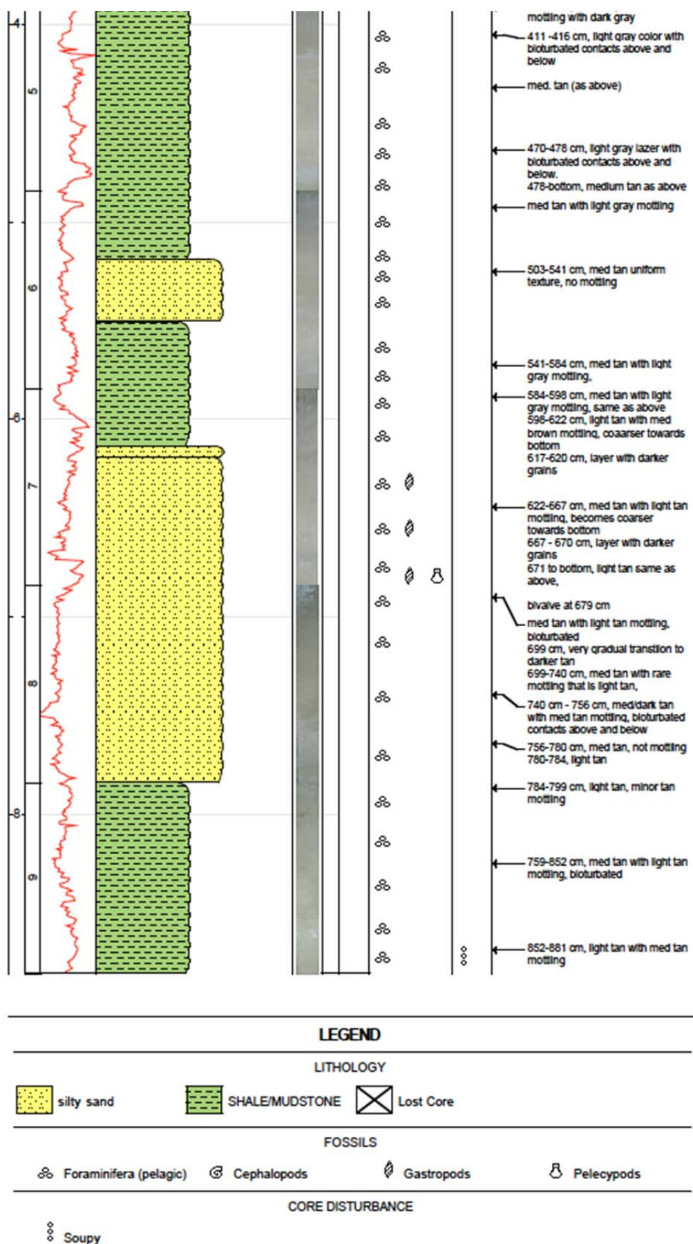
Fig. A11.1.8 Lithology log of core M94-482 Piston Core (by AppleCORE v10.2a).
