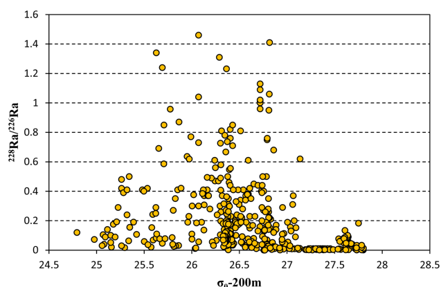
Figure 4. Surface water ^{228}\text{Ra}/^{226}\text{Ra} activity ratio versus potential density anomaly \sigma_0 at 200 m water depth. The data of \sigma_{0-200\text{ m}} are from Electronic Atlas of WOCE, while data of ^{228}\text{Ra}/^{226}\text{Ra} are the same as in Figure 2.
