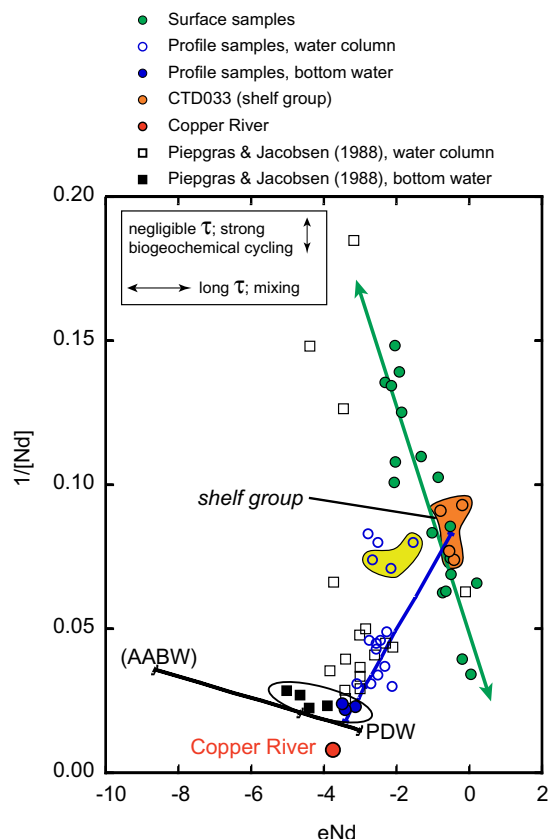
Fig. 8. Nd-isotope mixing plot. The black mixing line between PDW (Pacific Deep Water) and AABW (Antarctic Bottom Water) represents bottom water samples from Piepgras and Jacobsen (1988) (black squares). Note that no AABW was measured in this work. The blue line describes theoretical mixing of shelf/subsurface and abyssal waters (i.e., PDW). The green mixing line implies that the surface samples can all be explained by two-component mixing with a strong biogeochemical cycling. The three samples in yellow are from 100 m depth taken “in the wake” of an eddy. (For interpretation of the references to color in this figure legend, the reader is referred to the web version of this article.)
