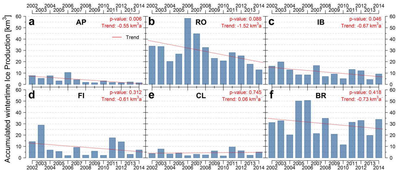
Fig. 17 Accumulated seasonal ice production [km 3 , IP] for the years from 2002 to 2014 during the winter period from April to September. The red line indicates the multi-year regional trend in km 3 /a. p value and numeric trend are stated in the top right corner for each sub-region (from Paul et al. 2015b)
