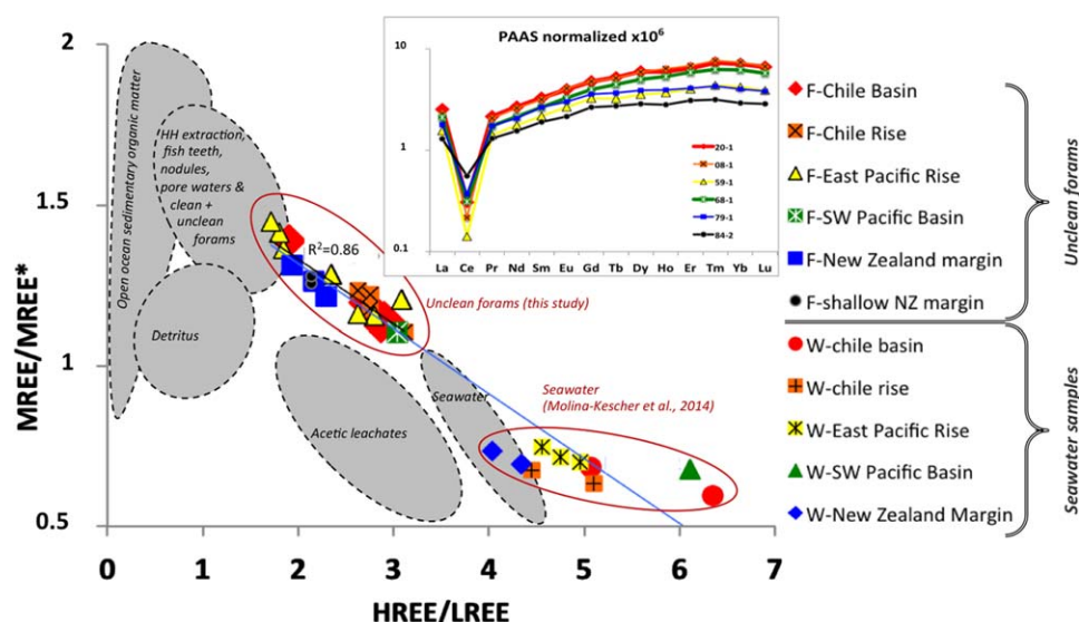
Figure 5. HREE/LREE (Tm+Yb+Lu/La+Pr+Nd) versus MREE/MREE* (Gd+Tb+Dy/LREE+HREE) of the REE concentrations normalized to Post-Achaean Australian Sedimentary Rocks (PAAS) [Taylor and McLennan, 1985] measured on “unclean” planktonic foraminifera samples of the different areas analyzed in this study (see legend: areas defined in Figure 3) and from seawater samples obtained for the same locations and depths [Molina-Kescher et al., 2014]. Shaded gray areas from Martin et al. [2010, and references therein], Kraft et al. [2013], and Freslon et al. [2014] are shown for comparison. PAAS normalized patterns from selected samples of each area are also presented in the smaller subplot.
