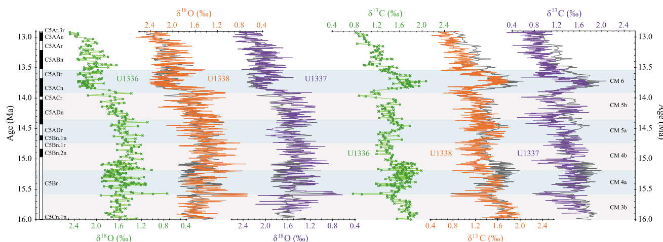
Figure 3. Comparison of benthic stable isotope time series of Site U1336 in green with U1337 in purple [Tian et al. , 2013] and U1338 in orange [Holbourn et al. , 2014]. Grey lines show the stable isotope record of Site U1336 overlapping with the ones of Sites U1337 and U1338 for direct comparison. The age of each stable isotope record is based on a different tuning approach, following the published age models for Sites U1337 [Tian et al. , 2013] and U1338 [Holbourn et al. , 2014]. Colored bands illustrate the carbon isotope maximum events (CM) of the Monterey Excursion (subdivisions by Holbourn et al. [2007]). The polarity stratigraphy of Site U1336 [Ohneiser et al. , 2013; Pälike et al. , 2010], based on the color reflectance b^* age model (see also Table S3), is provided for comparison.
