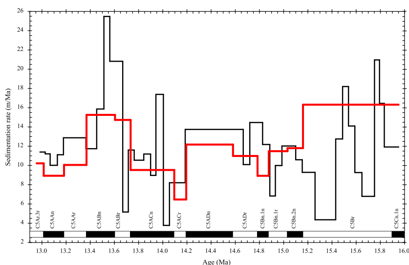
Figure 7. Comparison of the calculated sedimentation rates of Site U1336 based on the age model of color reflectance b* (black) and the age model derived from paleomagnetic data (red) [Ohneiser et al. , 2013]. The polarity stratigraphy of Site U1336, based on paleomagnetic data [Ohneiser et al. , 2013; Pälike et al. , 2010], is given for comparison.
